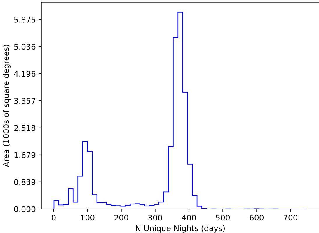
too_elab_r16_d2_ugrizy_v3.4_10yrs All sky all bands: N Unique Nights
