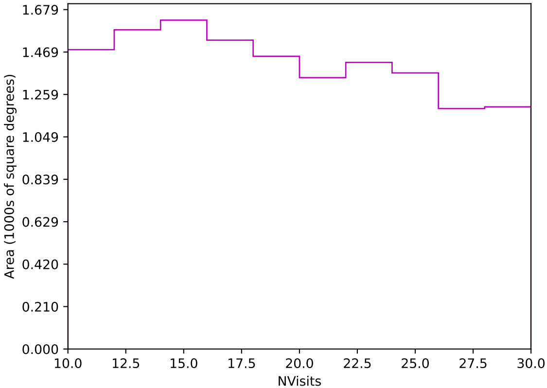
too_elab_r16_d2_ugrizy_v3.4_10yrs Yr 3-4 z band: NVisits
