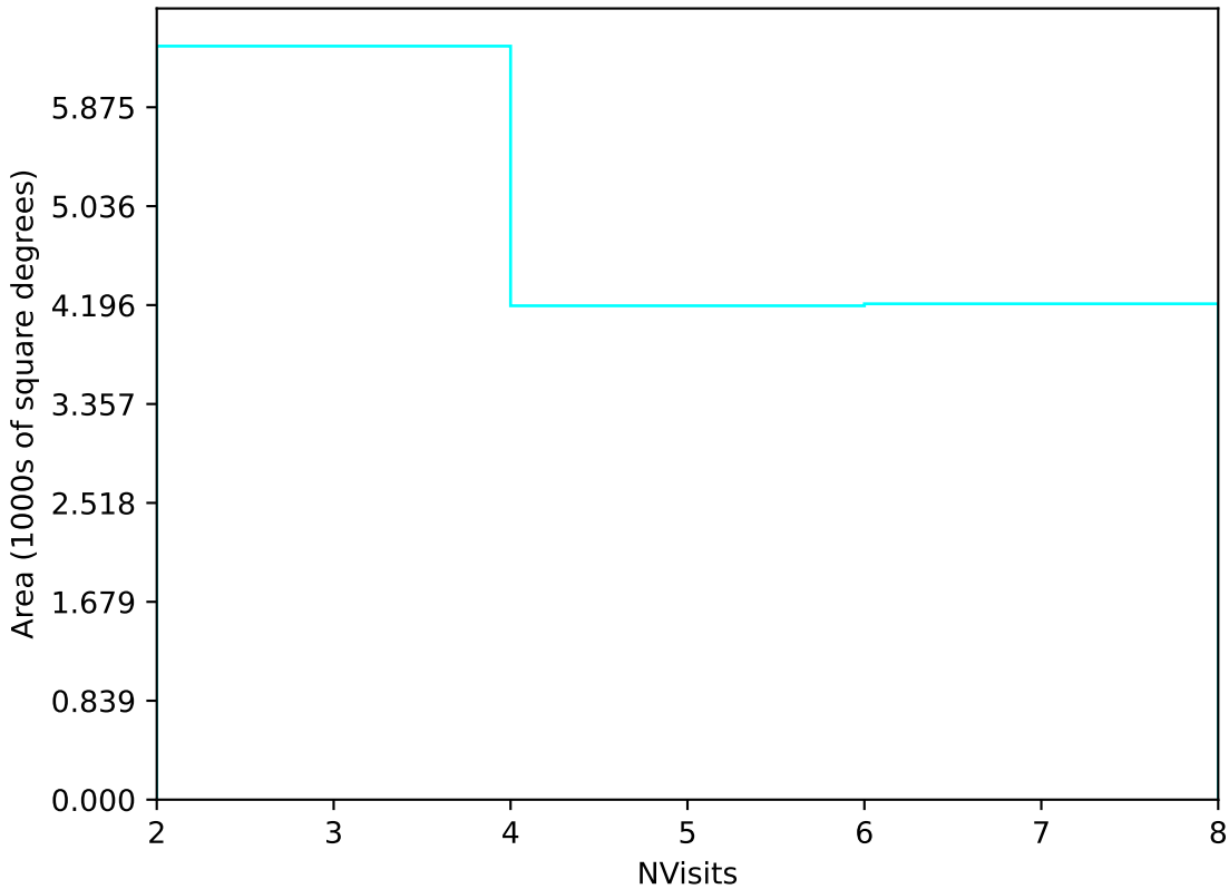
too_elab_r16_d2_ugrizy_v3.4_10yrs Yr 3-4 u band: NVisits
