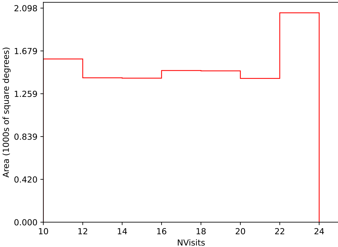
too_elab_r16_d2_ugrizy_v3.4_10yrs Yr 3-4 i band: NVisits
