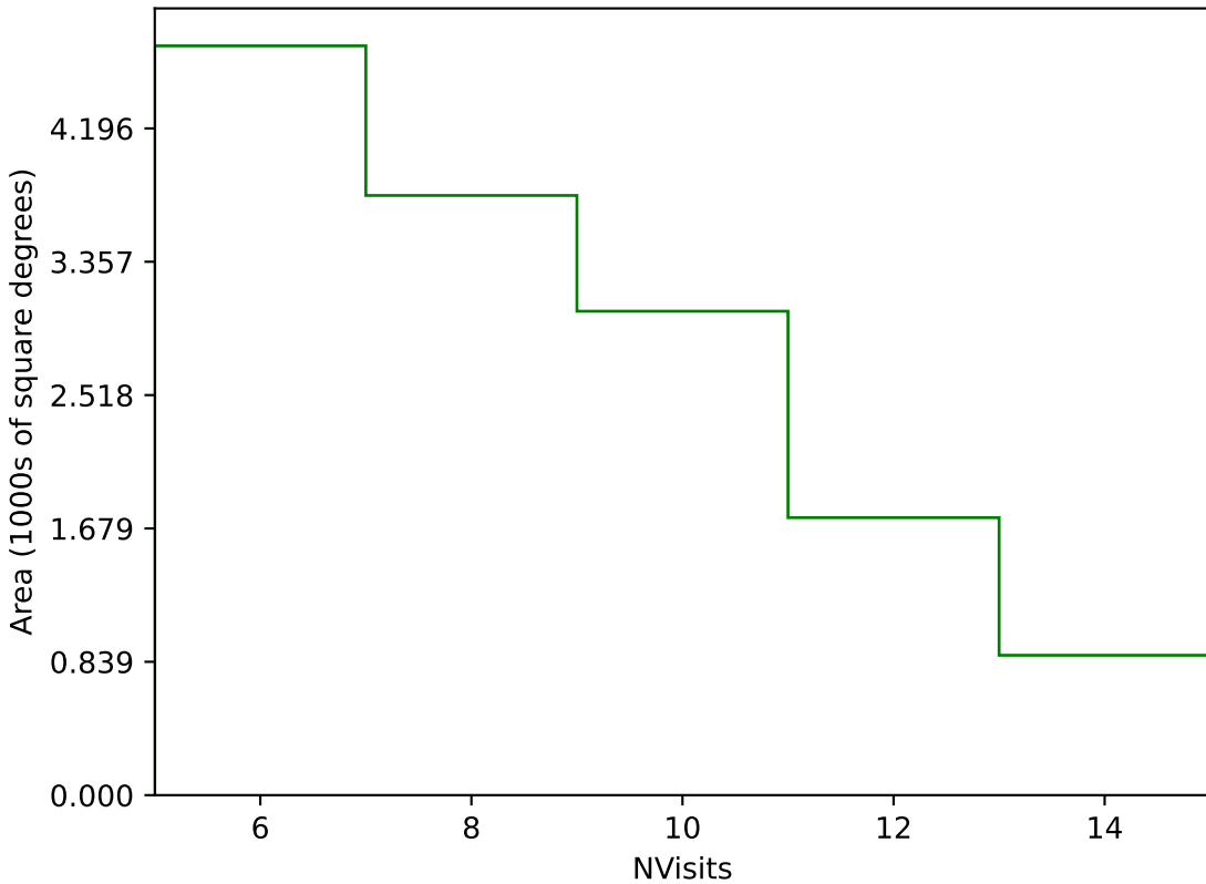
too_elab_r16_d2_ugrizy_v3.4_10yrs Yr 3-4 g band: NVisits
