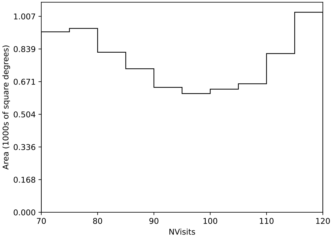
too_elab_r16_d2_ugrizy_v3.4_10yrs Yr 3-4 all bands: NVisits
