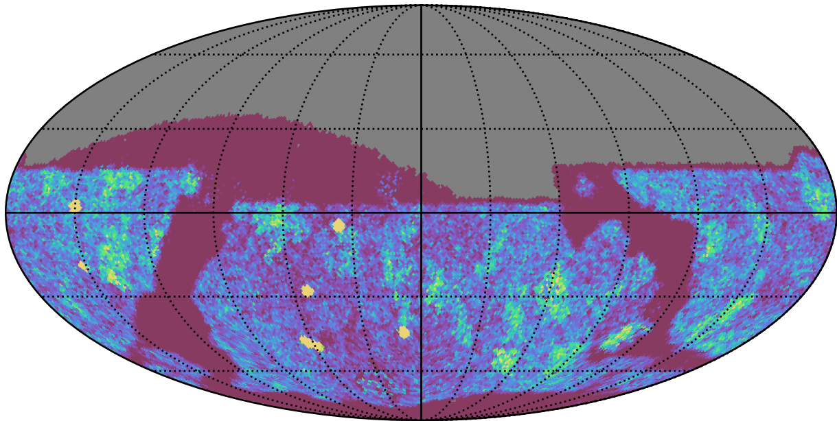
too_elab_r16_d2_ugrizy_v3.4_10yrs Yr 1 z band: NVisits
