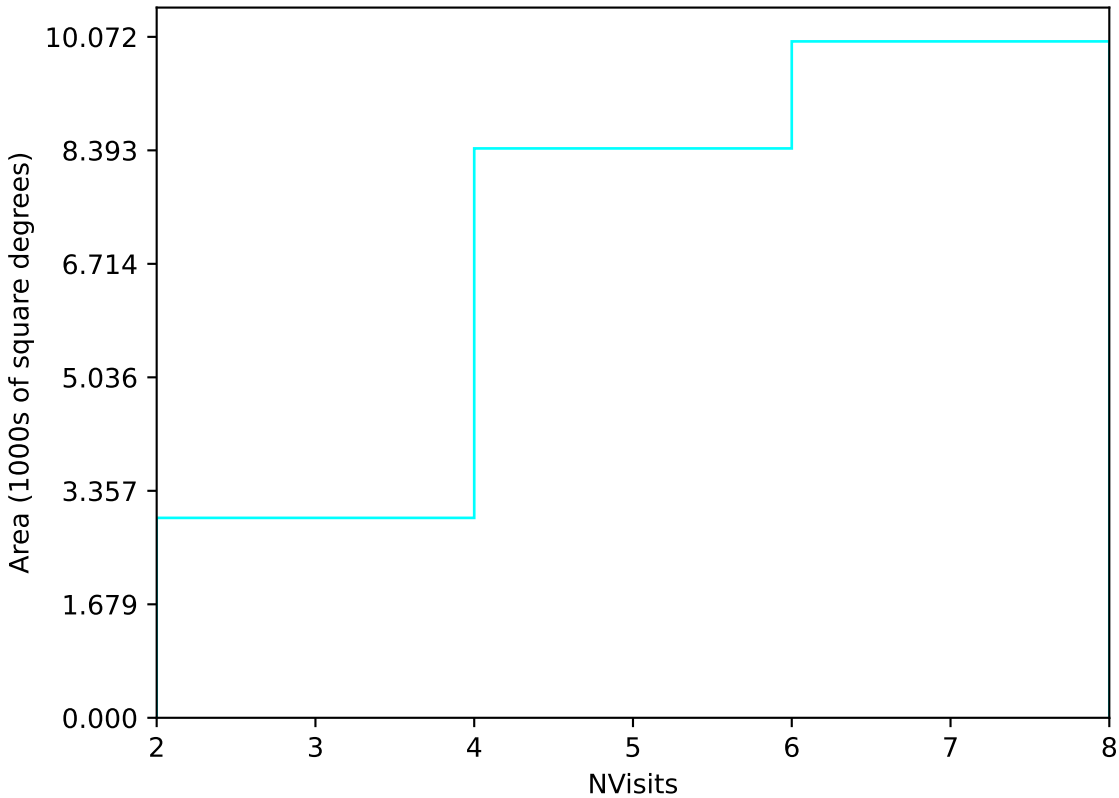
too_elab_r16_d2_ugrizy_v3.4_10yrs Yr 1 u band: NVisits
