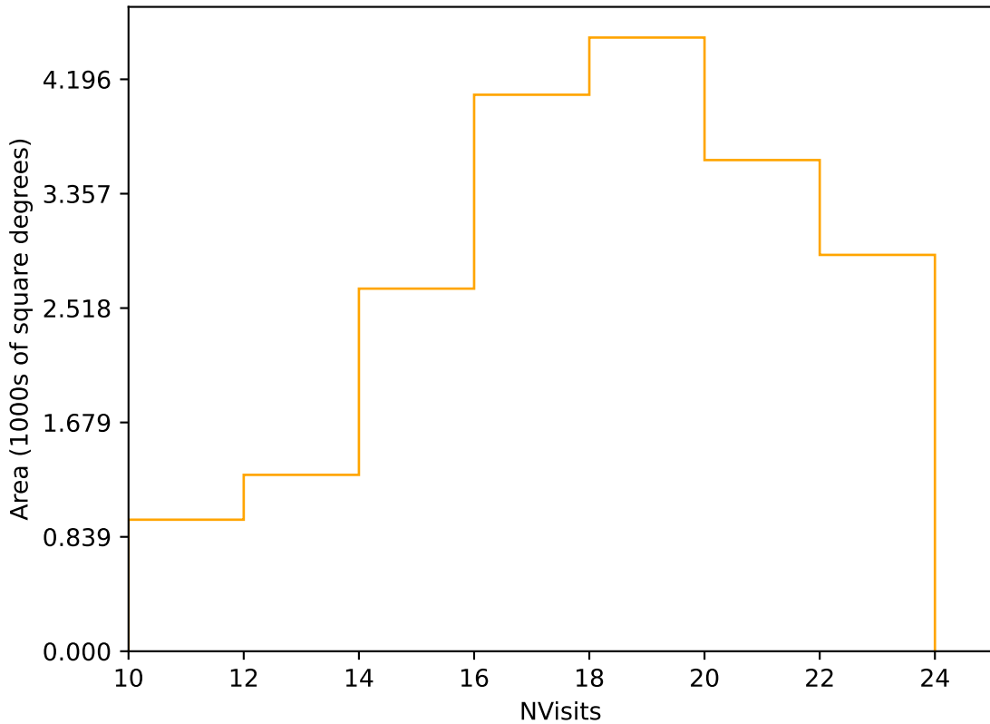
too_elab_r16_d2_ugrizy_v3.4_10yrs Yr 1 r band: NVisits
