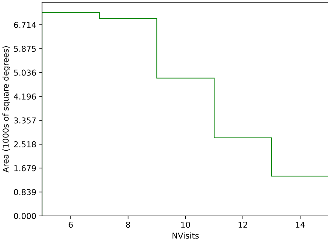
too_elab_r16_d2_ugrizy_v3.4_10yrs Yr 1 g band: NVisits
