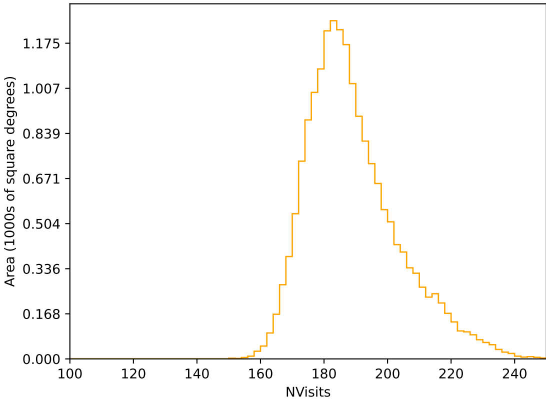
too_elab_r16_d2_ugrizy_v3.4_10yrs WFD r band: NVisits
