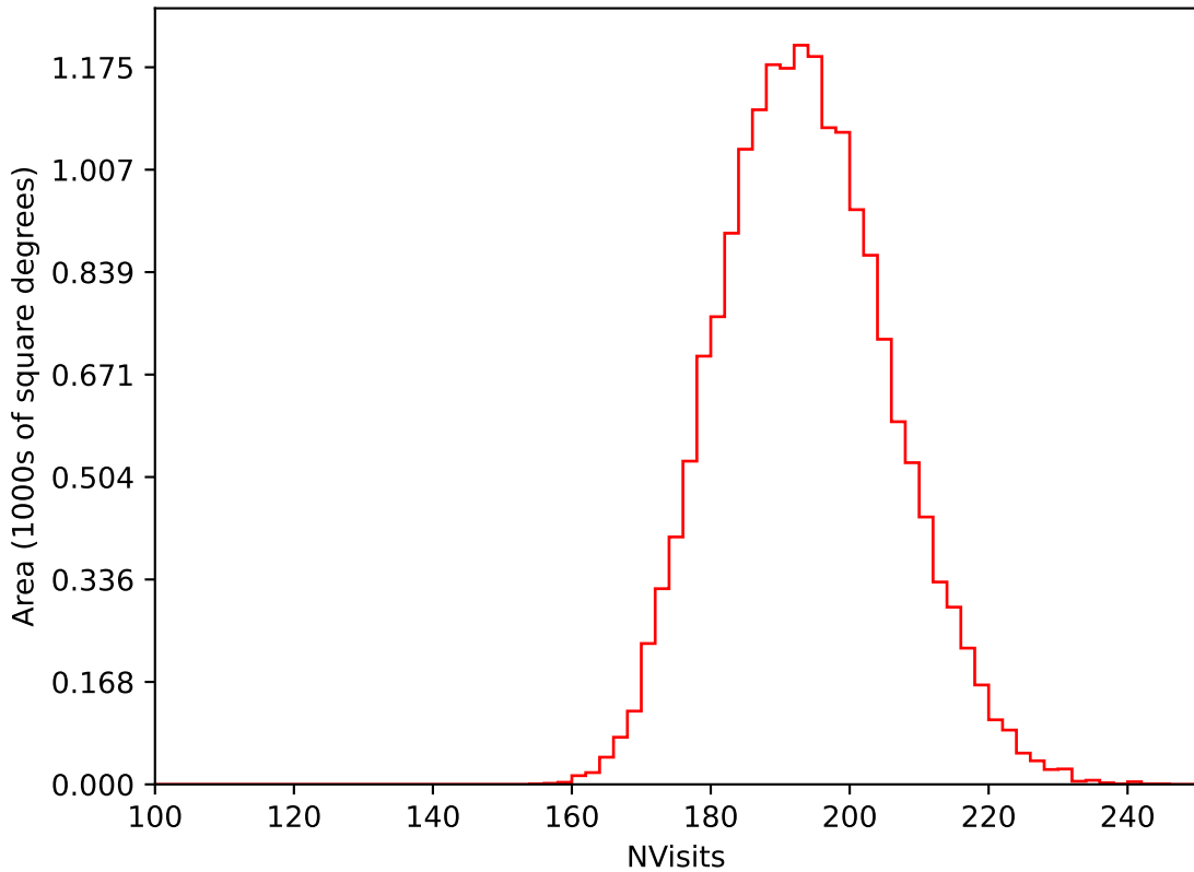
too_elab_r16_d2_ugrizy_v3.4_10yrs WFD i band: NVisits
