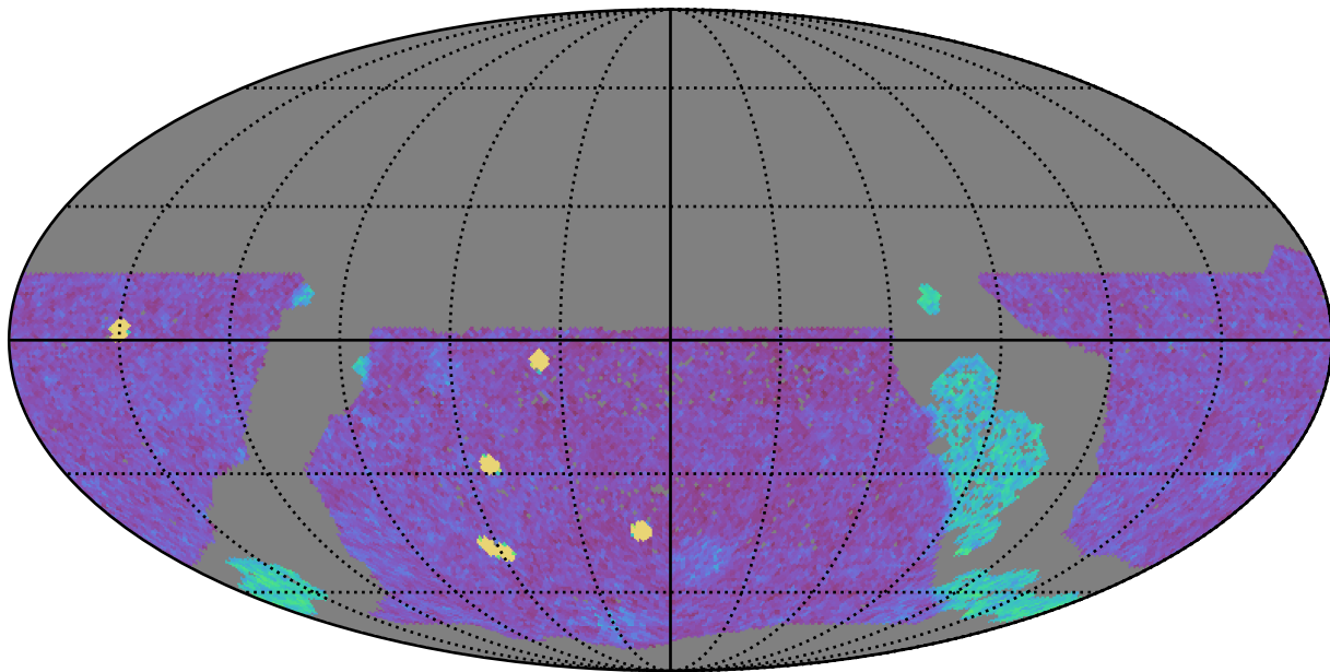
too_elab_r16_d2_ugrizy_v3.4_10yrs WFD g band: NVisits
