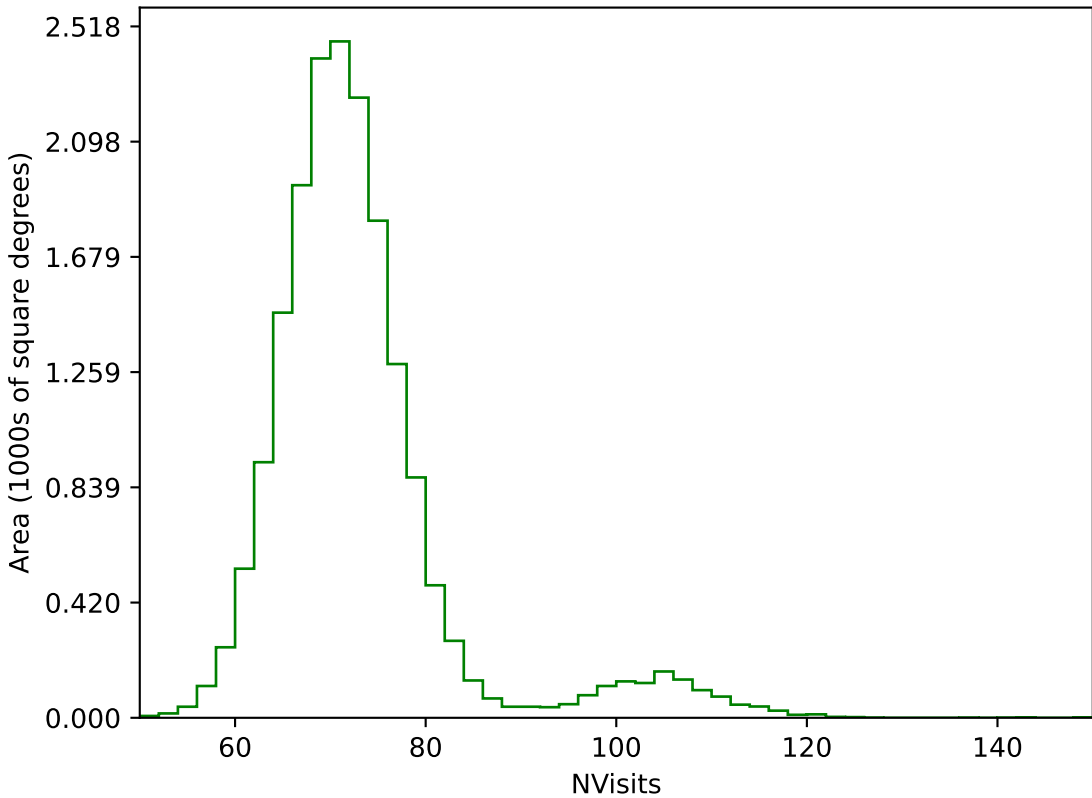
too_elab_r16_d2_ugrizy_v3.4_10yrs WFD g band: NVisits
