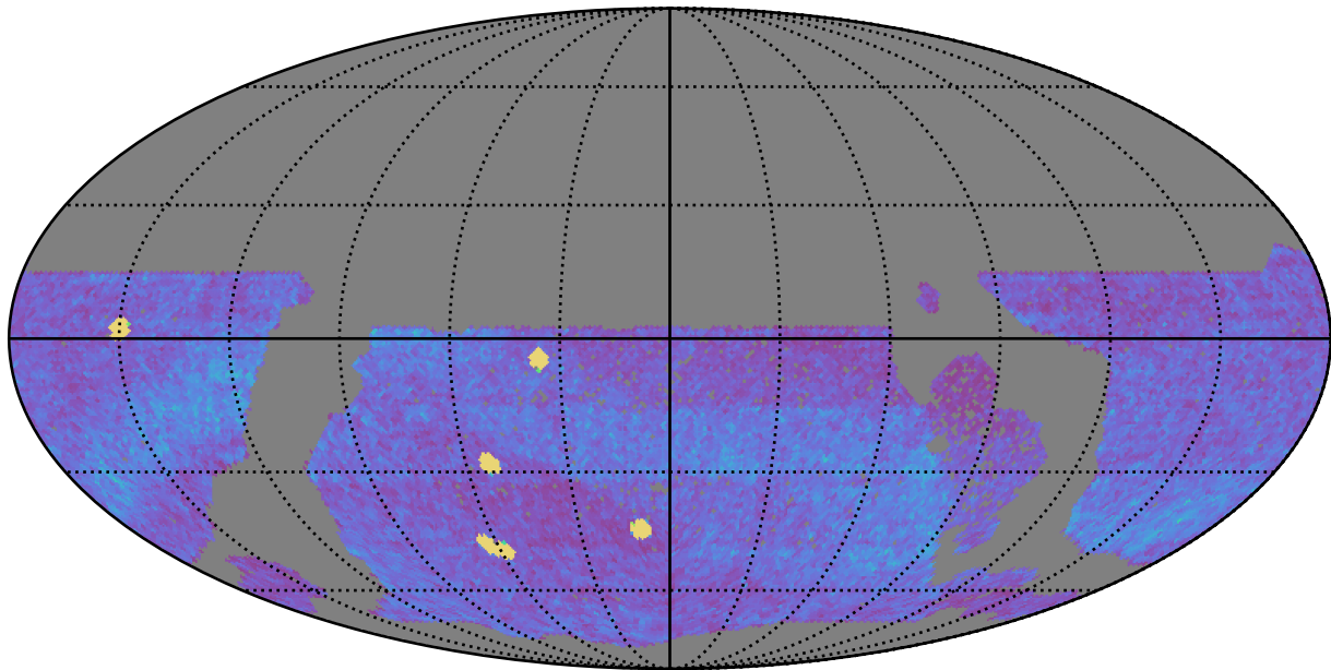
too_elab_r16_d2_ugrizy_v3.4_10yrs WFD all bands: NVisits
