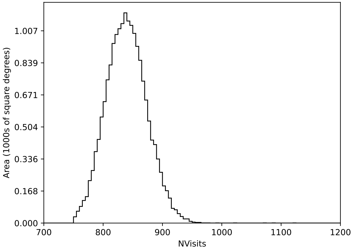
too_elab_r16_d2_ugrizy_v3.4_10yrs WFD all bands: NVisits
