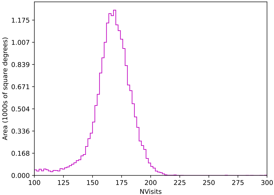
too_elab_r16_d2_ugrizy_v3.4_10yrs All sky z band: NVisits
