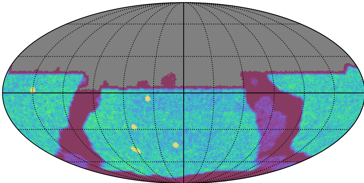
too_elab_r16_d2_ugrizy_v3.4_10yrs All sky u band: NVisits
