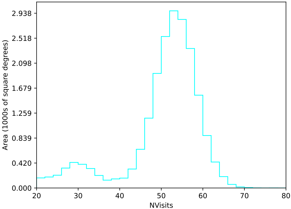
too_elab_r16_d2_ugrizy_v3.4_10yrs All sky u band: NVisits
