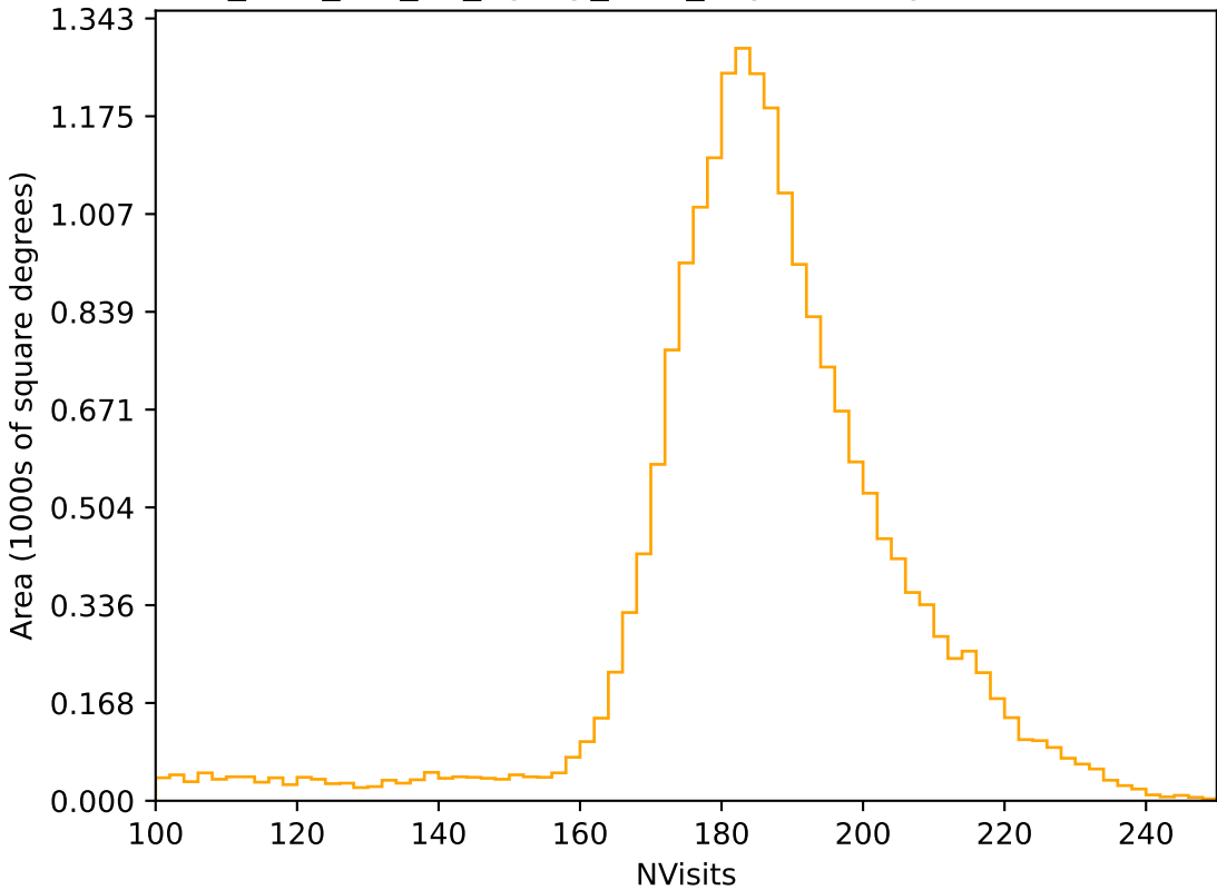
too_elab_r16_d2_ugrizy_v3.4_10yrs All sky r band: NVisits
