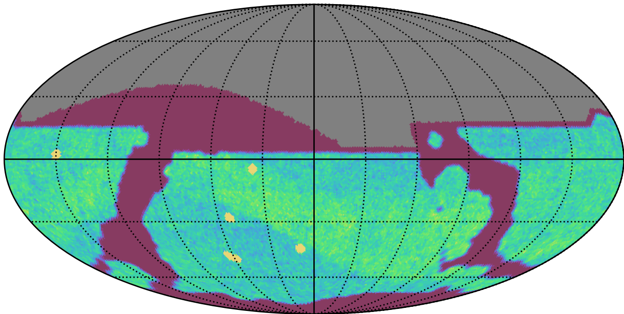
too_elab_r16_d2_ugrizy_v3.4_10yrs All sky i band: NVisits
