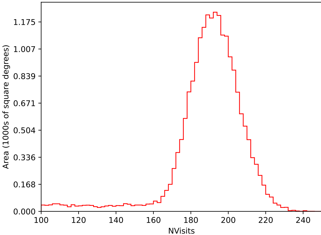
too_elab_r16_d2_ugrizy_v3.4_10yrs All sky i band: NVisits
