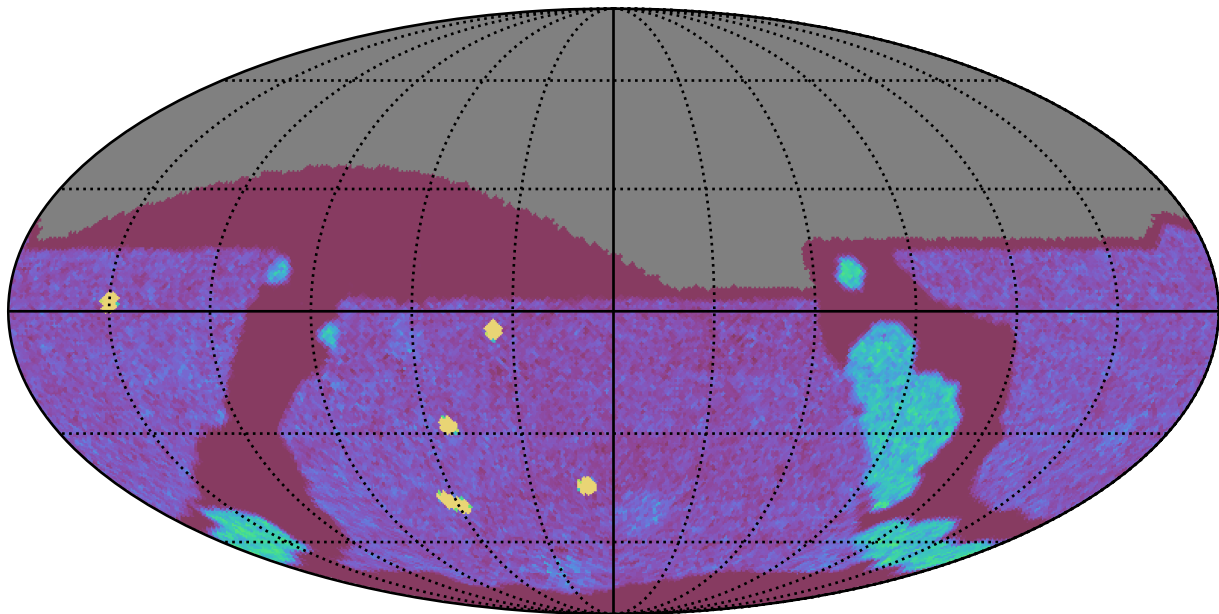
too_elab_r16_d2_ugrizy_v3.4_10yrs All sky g band: NVisits
