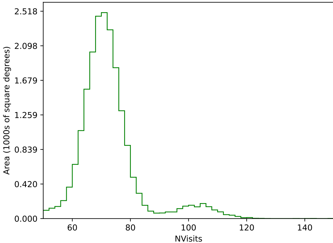
too_elab_r16_d2_ugrizy_v3.4_10yrs All sky g band: NVisits
