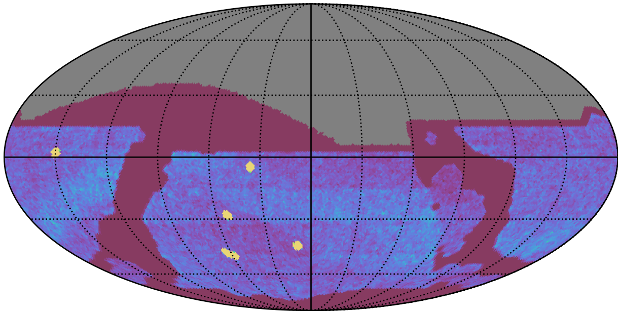
too_elab_r16_d2_ugrizy_v3.4_10yrs All sky all bands: NVisits
