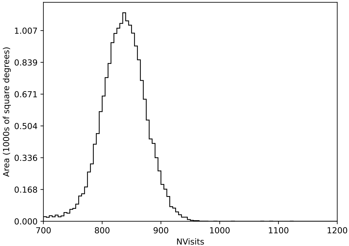
too_elab_r16_d2_ugrizy_v3.4_10yrs All sky all bands: NVisits
