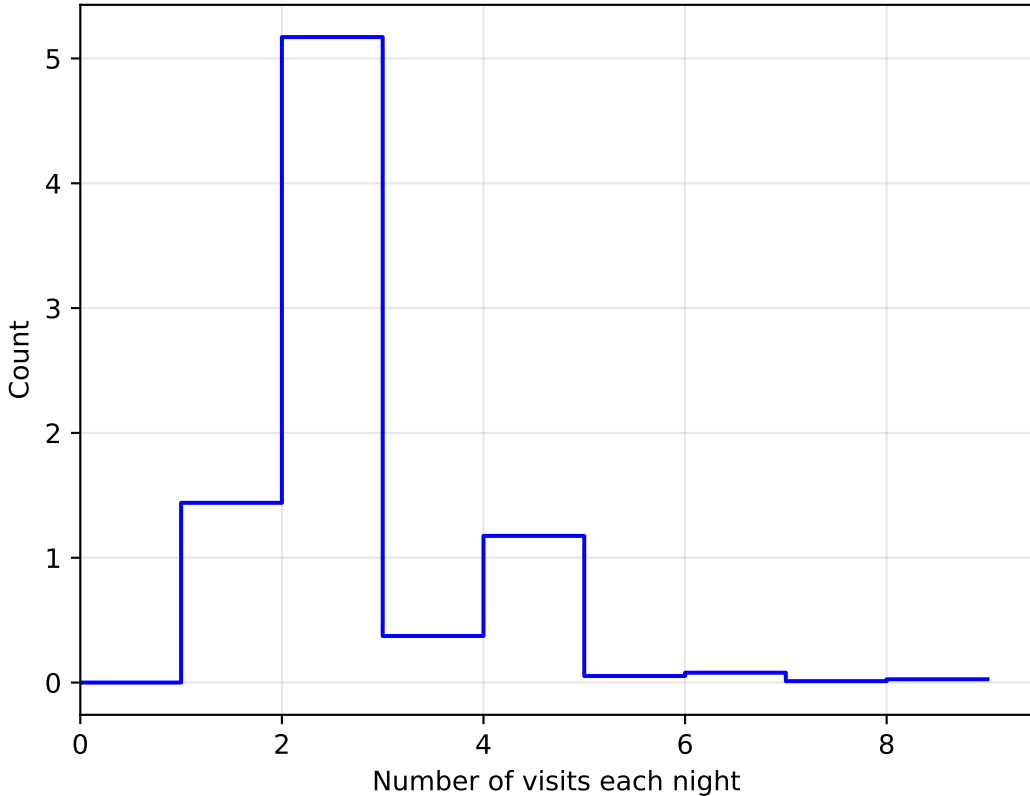
too_elab_r16_d2_ugrizy_v3.4_10yrs WFD: NVisitsPerNight 1e6
