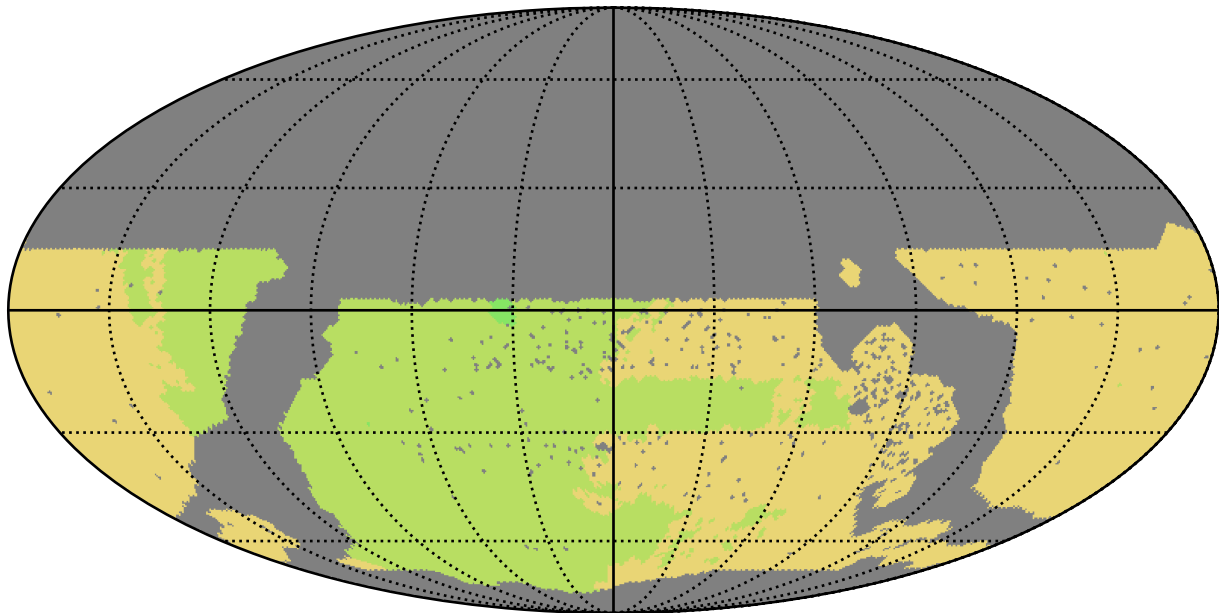
too_elab_r16_d2_ugrizy_v3.4_10yrs WFD all bands: NSeasons
