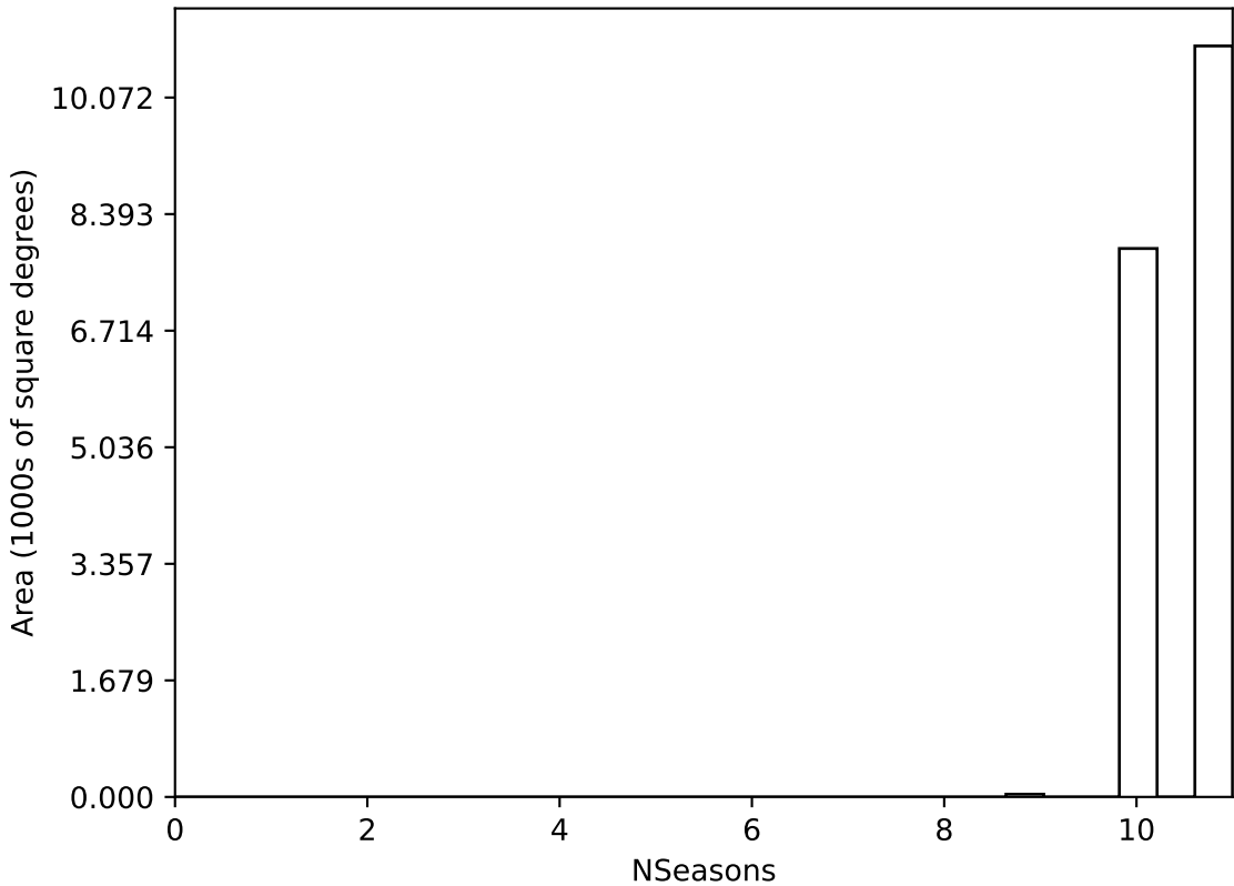
too_elab_r16_d2_ugrizy_v3.4_10yrs WFD all bands: NSeasons
