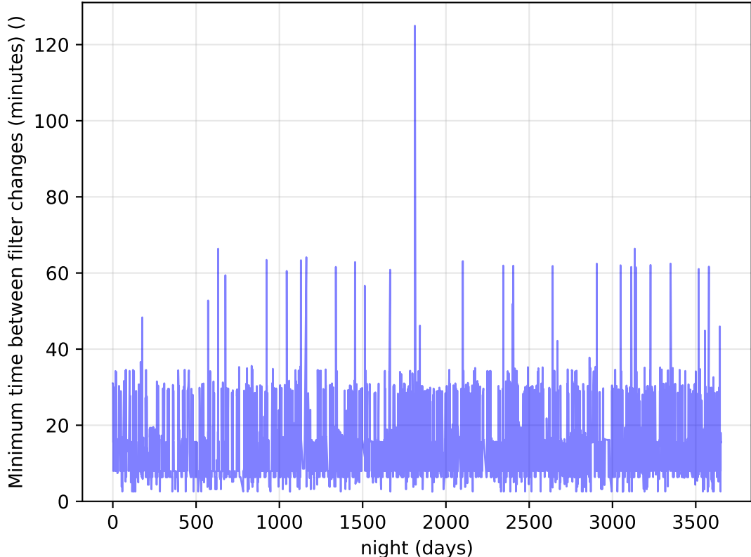
too_elab_r16_d2_ugrizy_v3.4_10yrs Per Night: Minimum time between filter changes (minutes)
