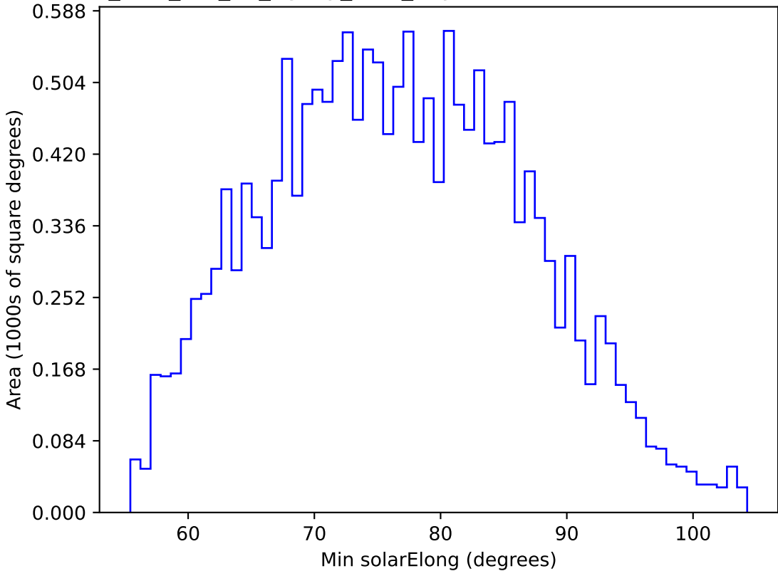
too_elab_r16_d2_ugrizy_v3.4_10yrs WFD u band: Min solarElong
