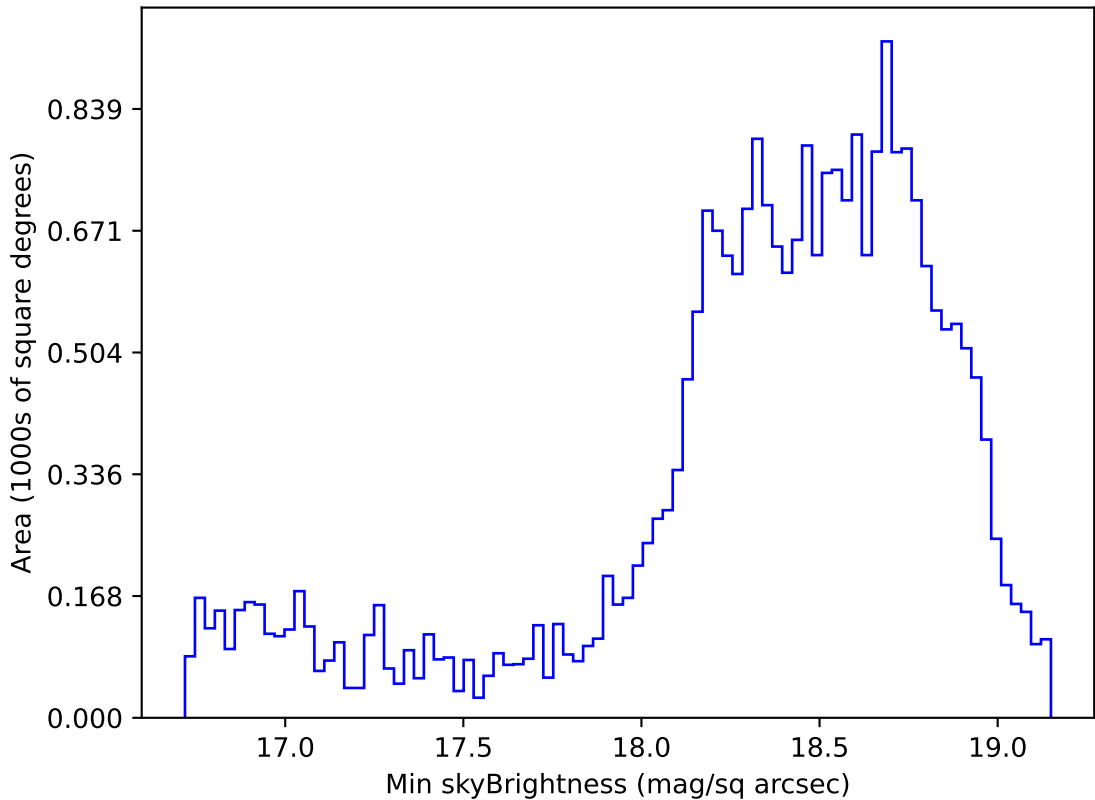
too_elab_r16_d2_ugrizy_v3.4_10yrs Yr 1 z band: Min skyBrightness
