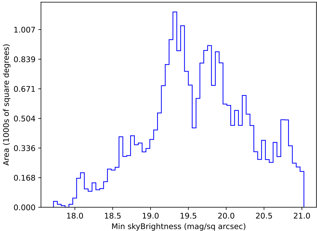
too_elab_r16_d2_ugrizy_v3.4_10yrs Yr 1 r band: Min skyBrightness
