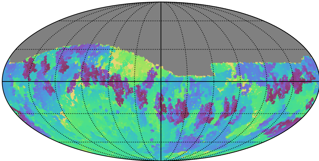
too_elab_r16_d2_ugrizy_v3.4_10yrs Yr 1 i band: Min skyBrightness
