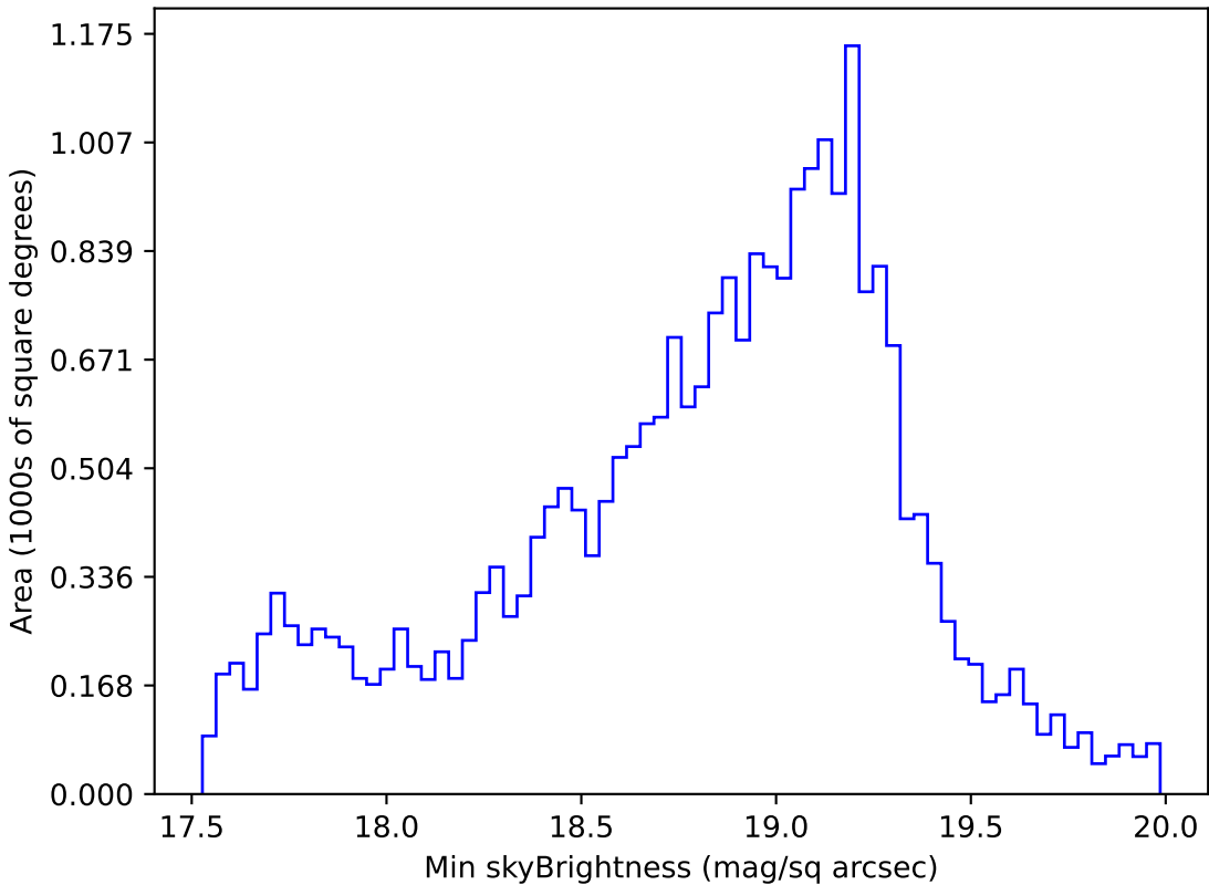
too_elab_r16_d2_ugrizy_v3.4_10yrs Yr 1 i band: Min skyBrightness
