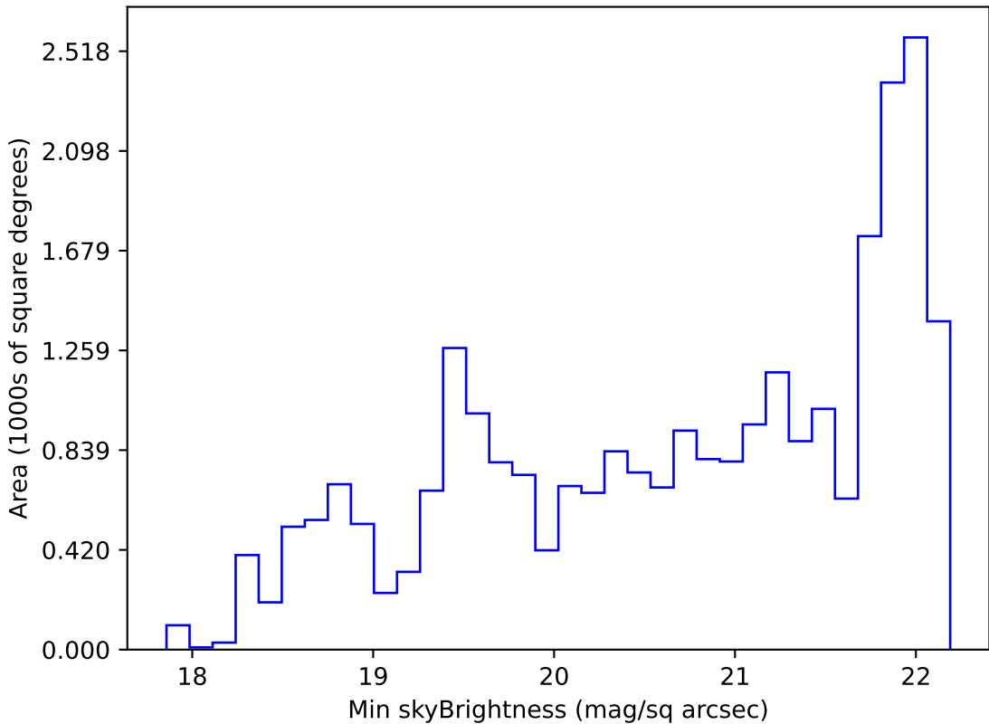
too_elab_r16_d2_ugrizy_v3.4_10yrs Yr 1 g band: Min skyBrightness
