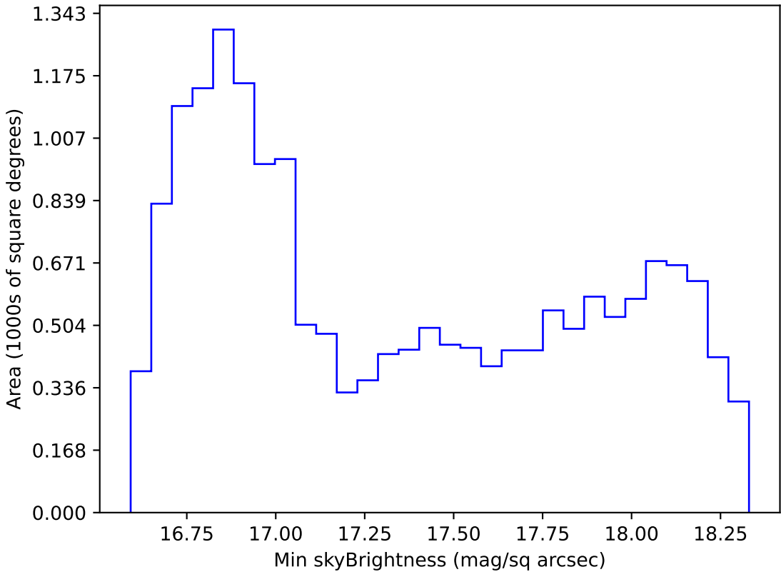
too_elab_r16_d2_ugrizy_v3.4_10yrs WFD z band: Min skyBrightness
