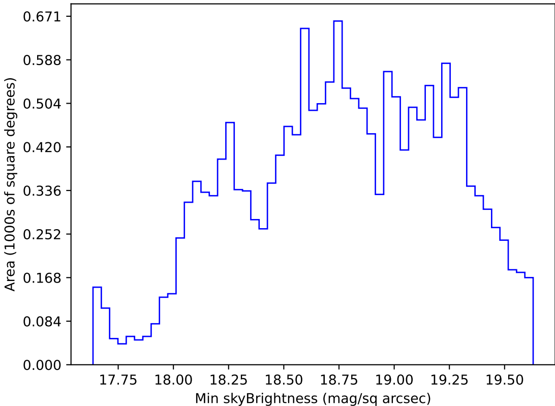
too_elab_r16_d2_ugrizy_v3.4_10yrs WFD r band: Min skyBrightness
