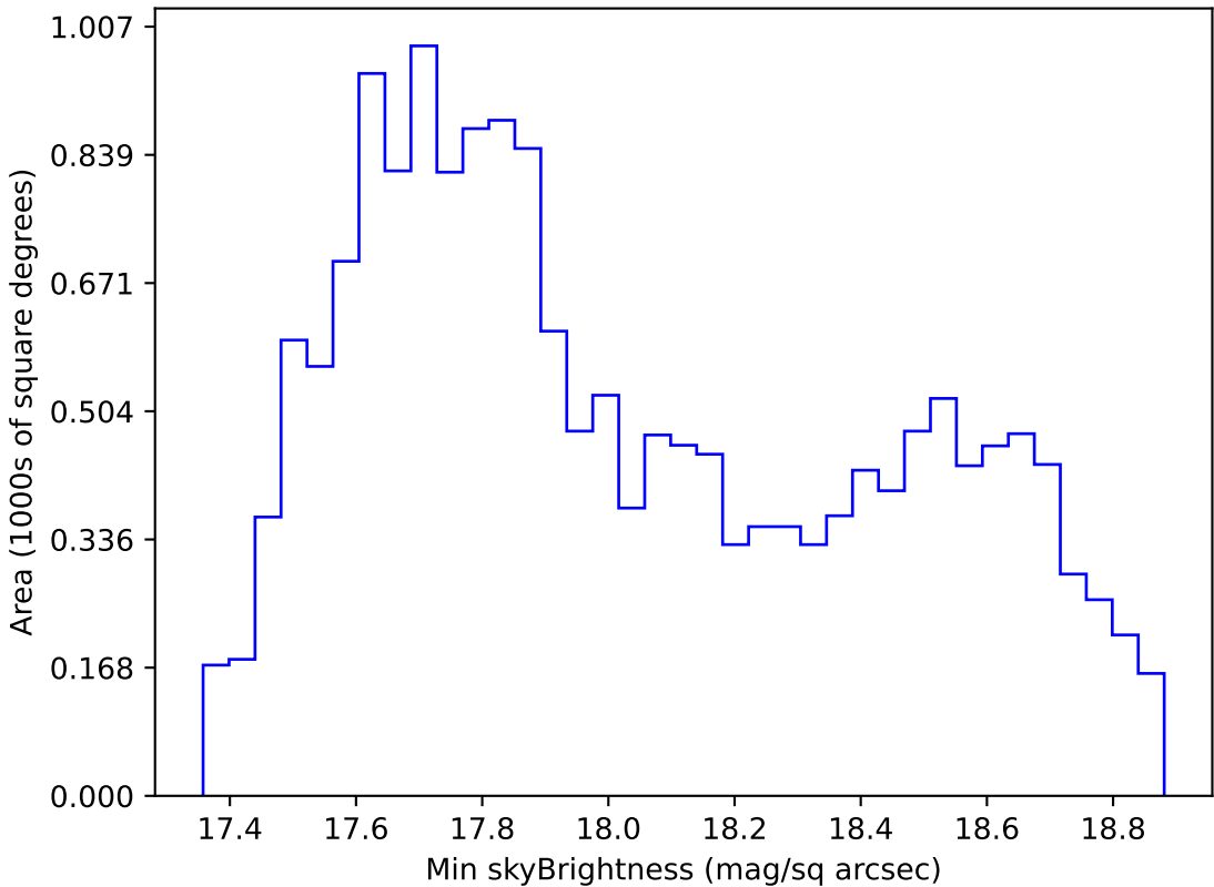
too_elab_r16_d2_ugrizy_v3.4_10yrs WFD i band: Min skyBrightness
