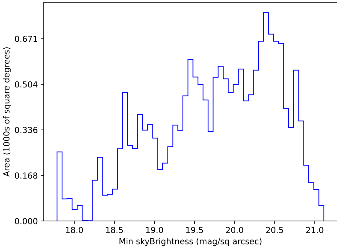
too_elab_r16_d2_ugrizy_v3.4_10yrs WFD g band: Min skyBrightness
