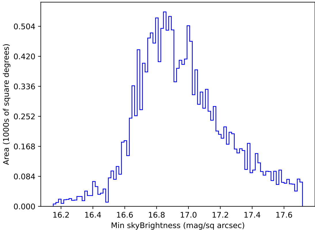
too_elab_r16_d2_ugrizy_v3.4_10yrs WFD all bands: Min skyBrightness
