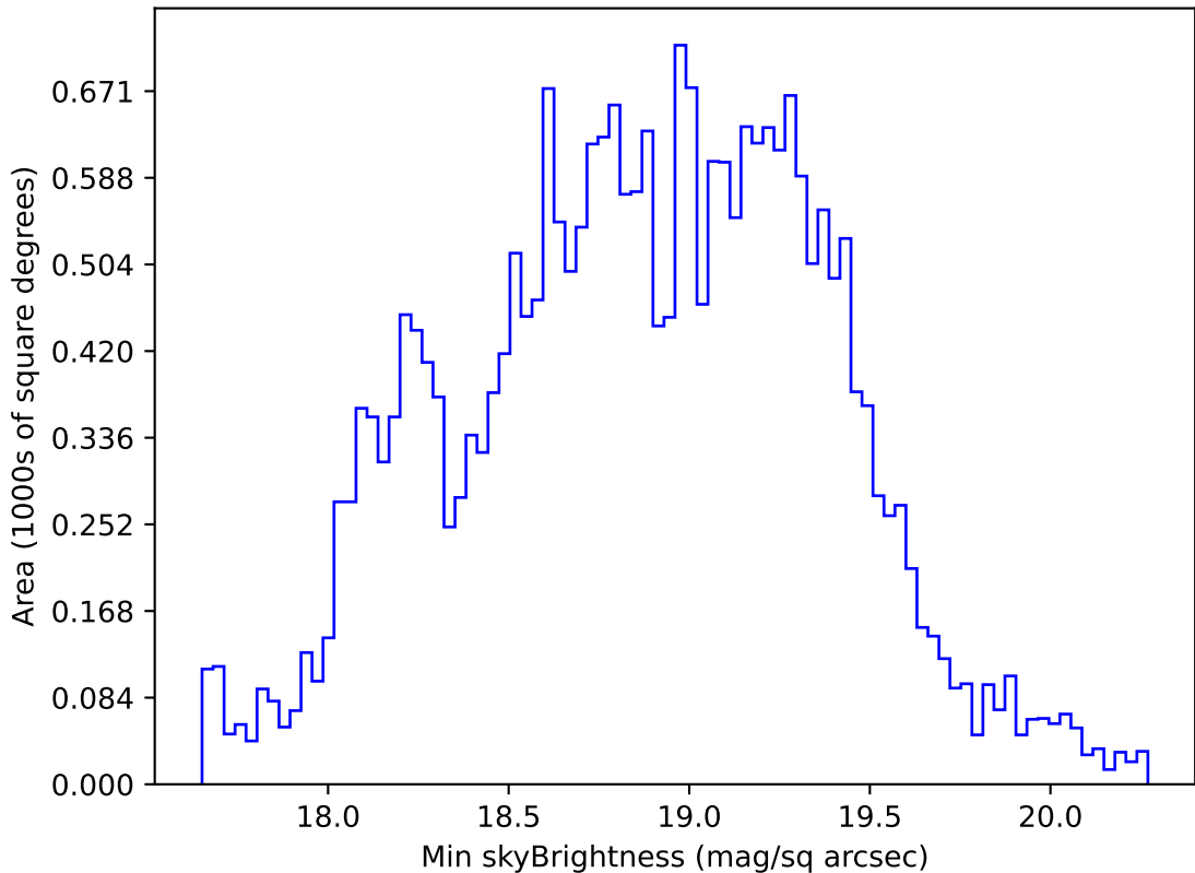
too_elab_r16_d2_ugrizy_v3.4_10yrs All sky r band: Min skyBrightness
