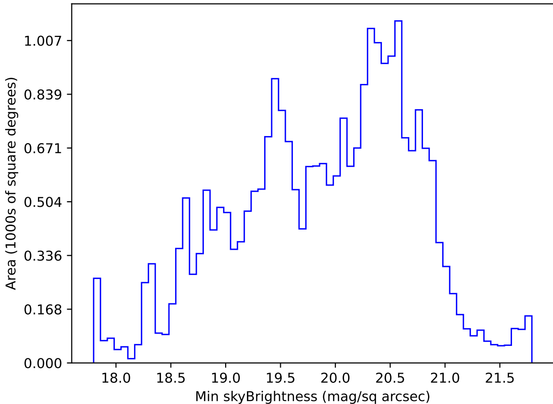
too_elab_r16_d2_ugrizy_v3.4_10yrs All sky g band: Min skyBrightness
