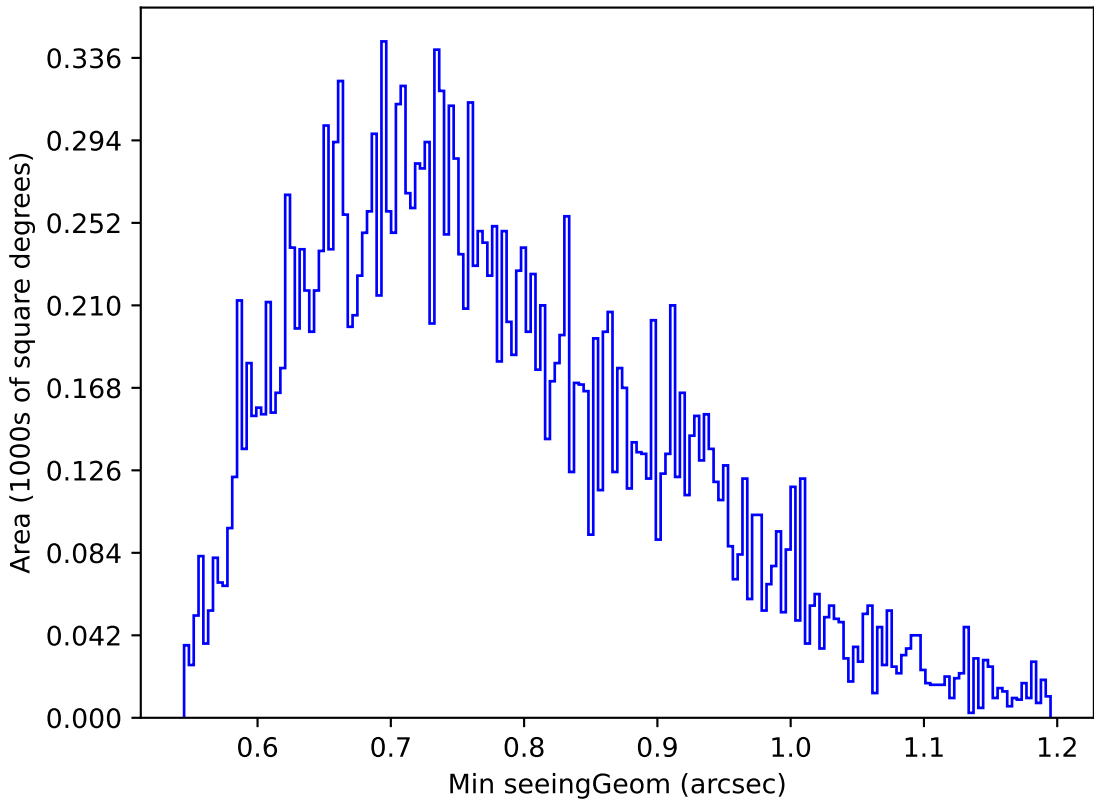
too_elab_r16_d2_ugrizy_v3.4_10yrs Yr 1 u band: Min seeingGeom
