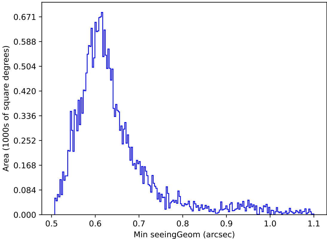
too_elab_r16_d2_ugrizy_v3.4_10yrs Yr 1 r band: Min seeingGeom
