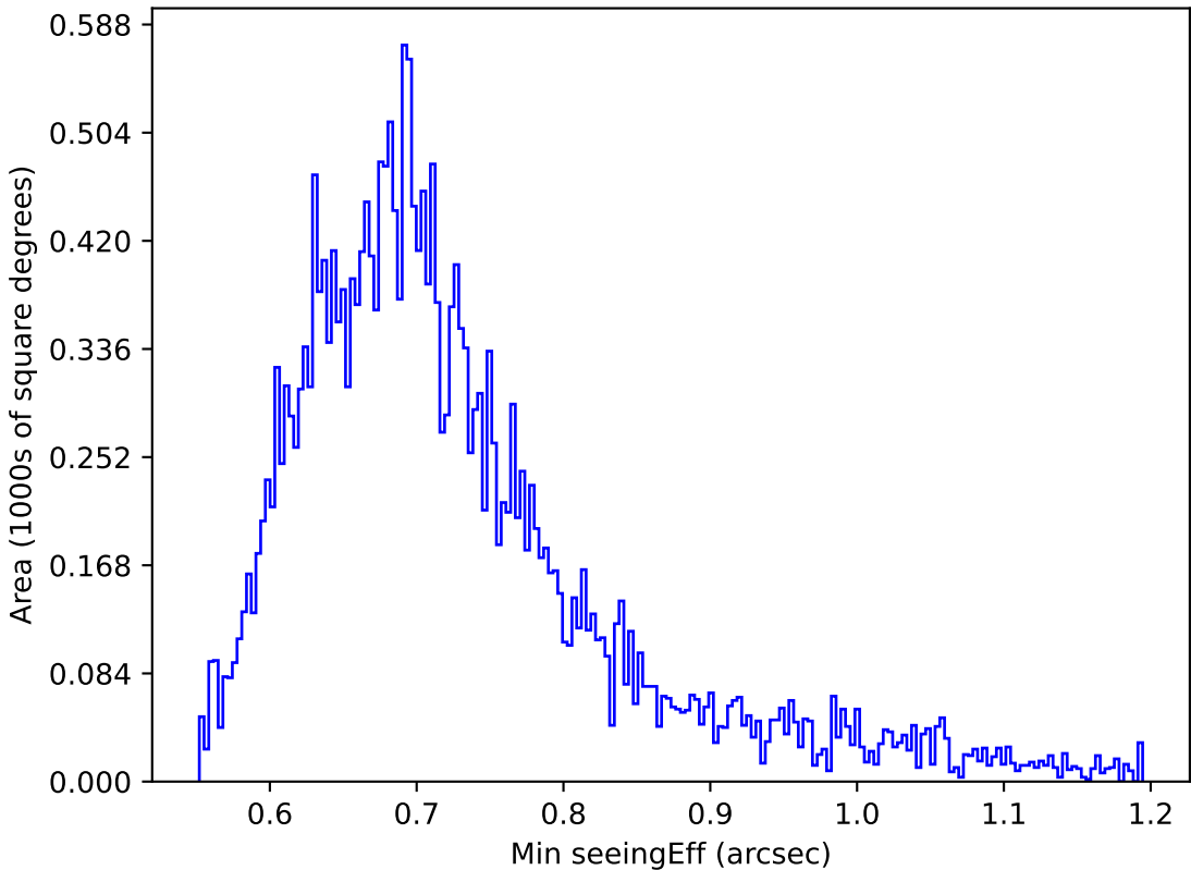
too_elab_r16_d2_ugrizy_v3.4_10yrs Yr 1 z band: Min seeingEff
