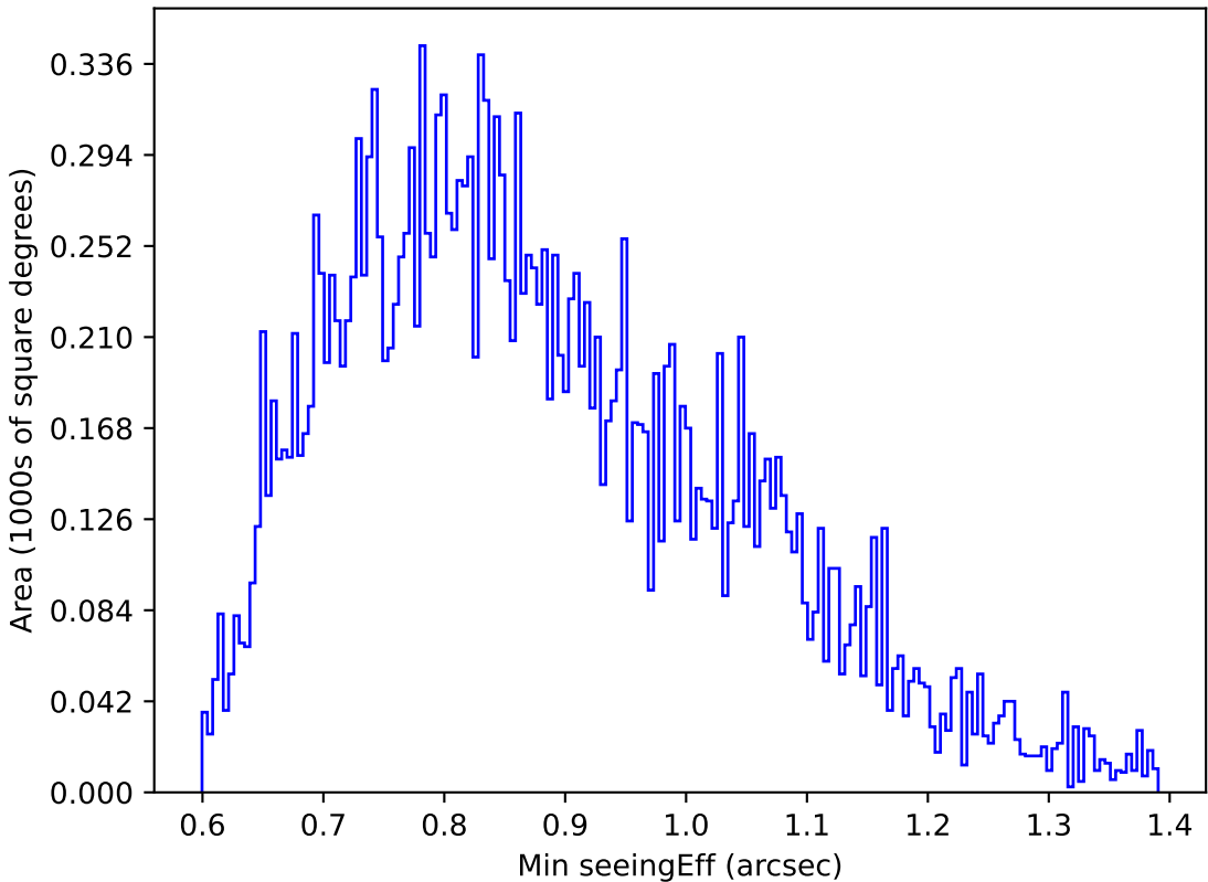
too_elab_r16_d2_ugrizy_v3.4_10yrs Yr 1 u band: Min seeingEff
