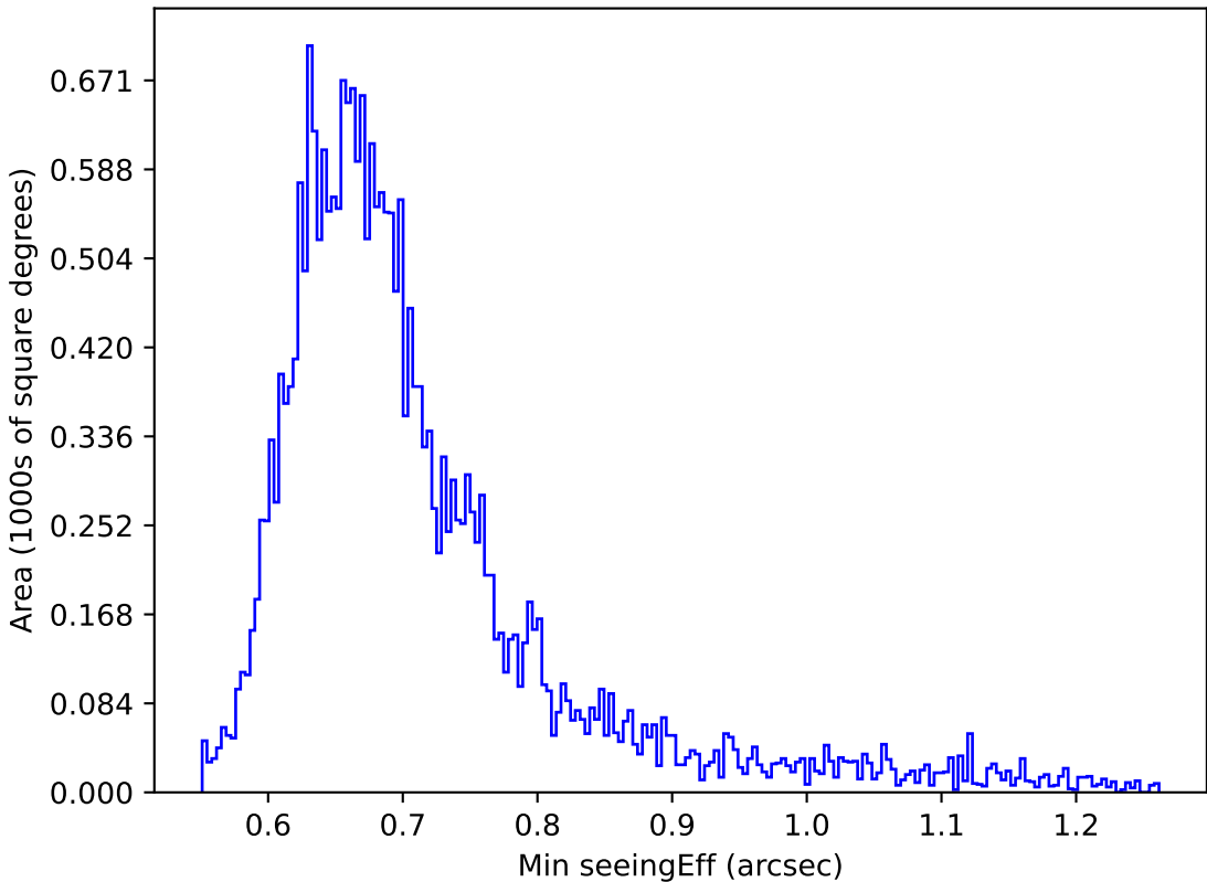
too_elab_r16_d2_ugrizy_v3.4_10yrs Yr 1 i band: Min seeingEff
