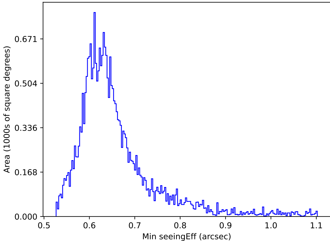
too_elab_r16_d2_ugrizy_v3.4_10yrs Yr 1 all bands: Min seeingEff
