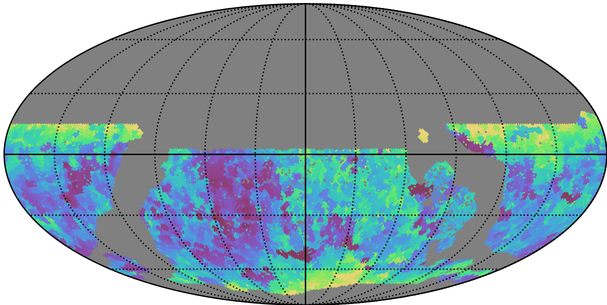
too_elab_r16_d2_ugrizy_v3.4_10yrs WFD i band: Min seeingEff
